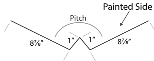
VALLEY FLASHING
