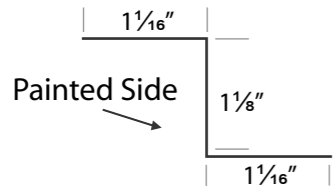
ZEE CLOSURE
