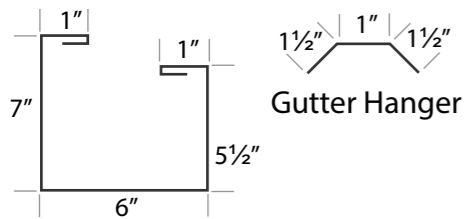
HR GUTTER
