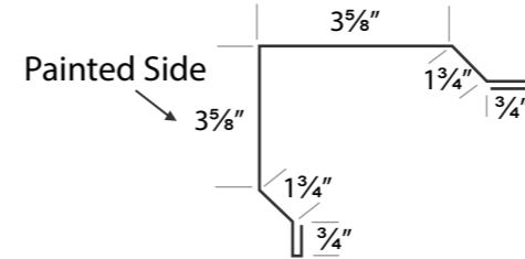
HR OUTSIDE CORNER
