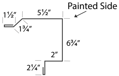
LONG EAVE TRIM
