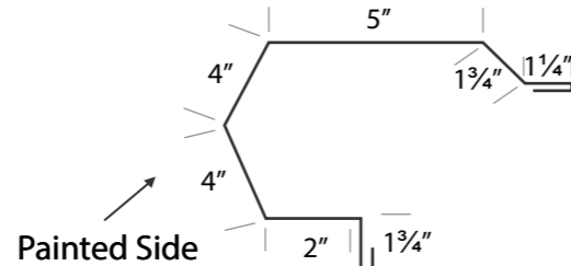
HR GABLE
