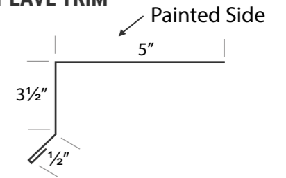
SHORT EAVE TRIM
