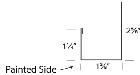
HR J-CHANNEL
