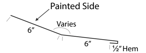
HR DOUBLE ANGLE
