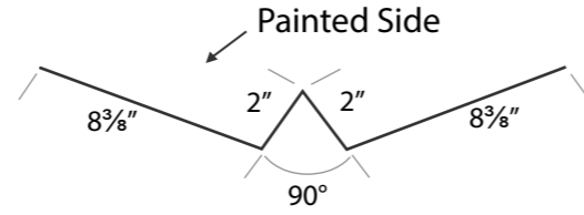
HR INSIDE CORNER
