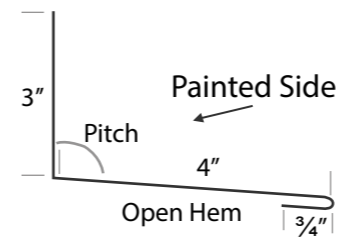
OPEN HEM SIDEWALL / ENDWALL
