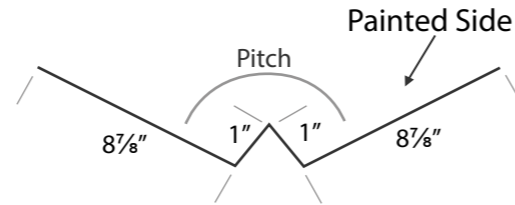
VALLEY FLASHING
