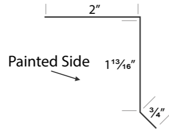
CLEAT
