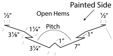
OPEN HEM VALLEY
