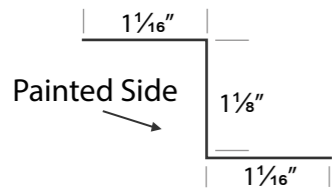
ZEE CLOSURE
