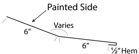
OPEN HEM TRANSITION
