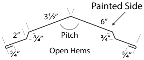
OPEN HEM RIDGECAP
