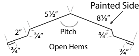
OPEN HEM WIDE RIDGECAP
