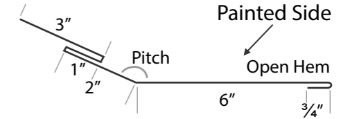
BULLNOSE TRANSITION
