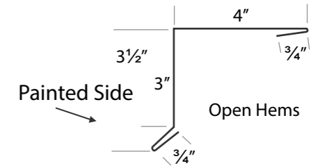
OPEN HEM GABLE
